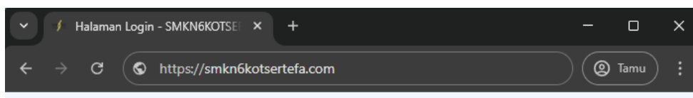
Gambar 1.1 Address Bar
