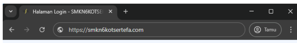
Gambar 4.1 Address Bar
