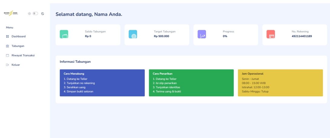
Gambar 4.3 Halaman Dashboard
